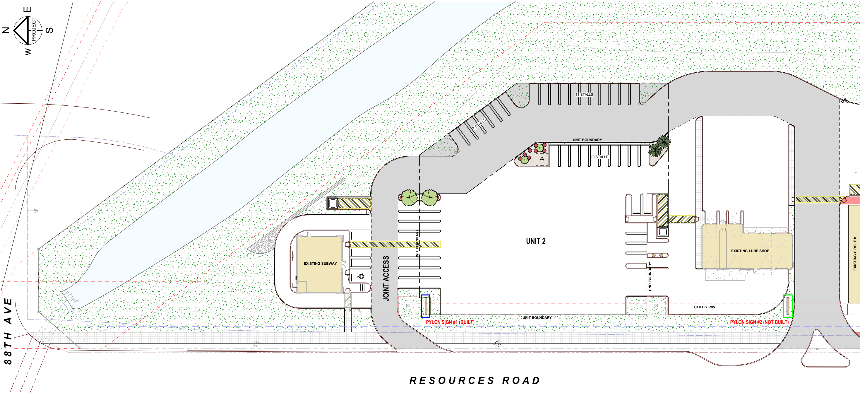
① UNIT 2 SITE LAYOUT 1" = 50'-0"
